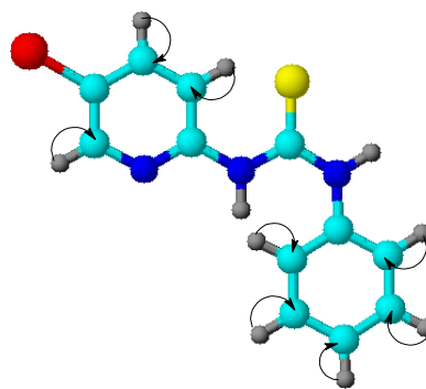
Figure 2. Correlation of HMQC ( ^1\text{H} - ^{13}\text{C} ) of compound 6
